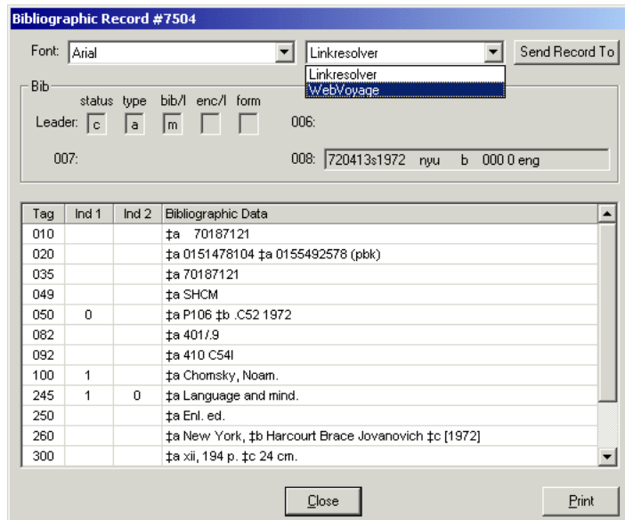
Figure 4-22. Send Record To button and drop-down as seen in the Acquisitions and Circulation modules
